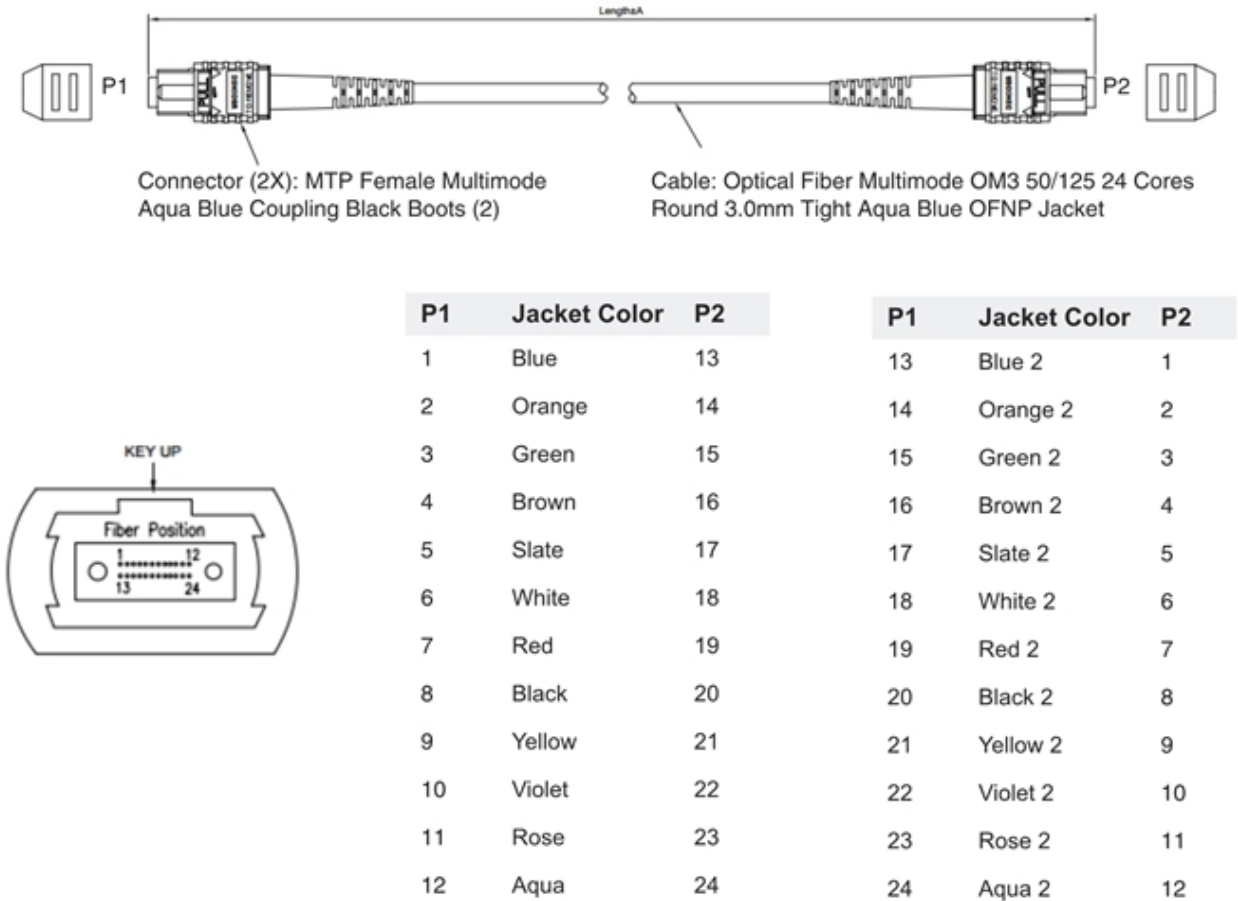
Figure 20 MPO/MTP 24 Position Fiber Cable
